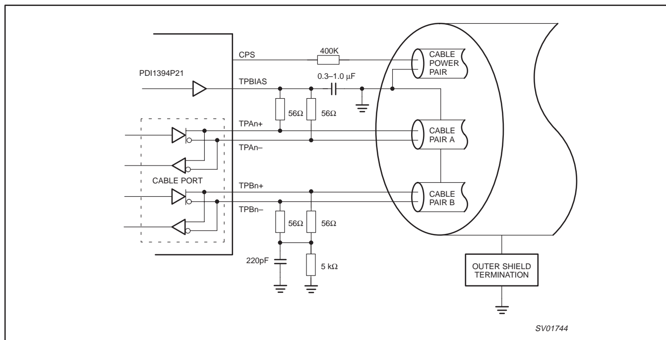
Figure 4. Twisted pair cable interface connections
