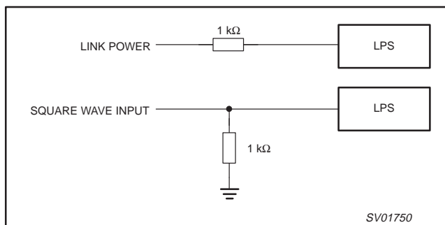
Figure 7. Non-isolated connection variations for LPS
