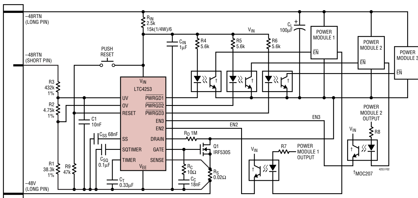
Figure 2. -48V/2.5A Application with a Wider Operating Range
