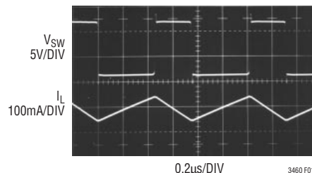
Switching Waveforms
