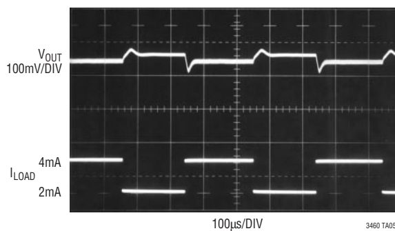
Load Step Response
