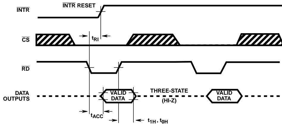
FIGURE 10B. OUTPUT ENABLE AND RESET \text{INTR}
