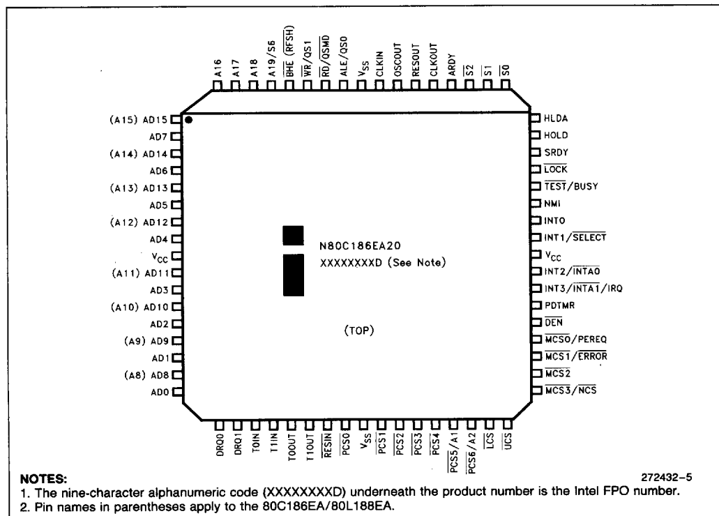
Figure 5. 68-Lead PLCC Pinout Diagram
