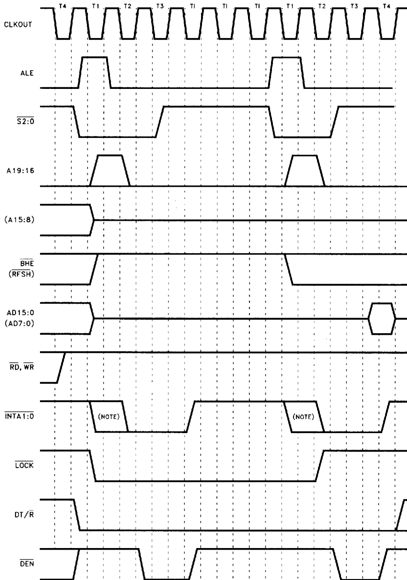
Figure 20. \overline{\text{INTA}} Cycle Waveform
