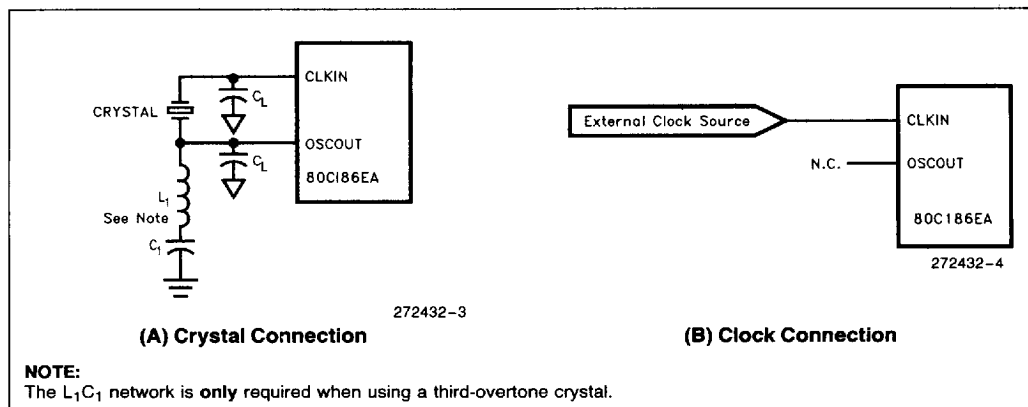
Figure 2. Clock Configurations
