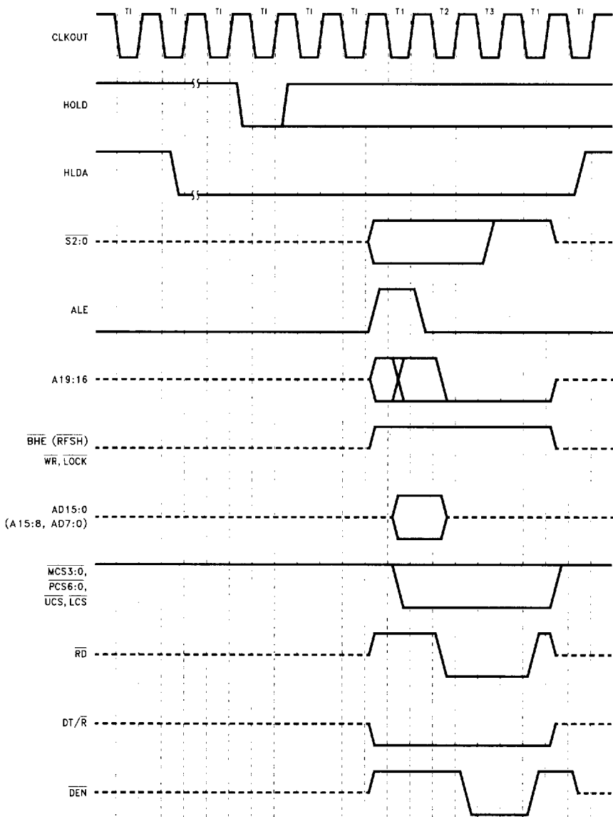
Figure 22. DRAM Refresh Cycle During Hold Acknowledge
