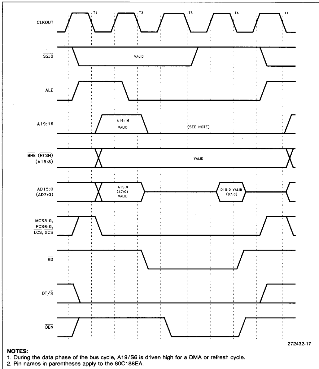
Figure 17. Read, Fetch and Refresh Cycle Waveform
