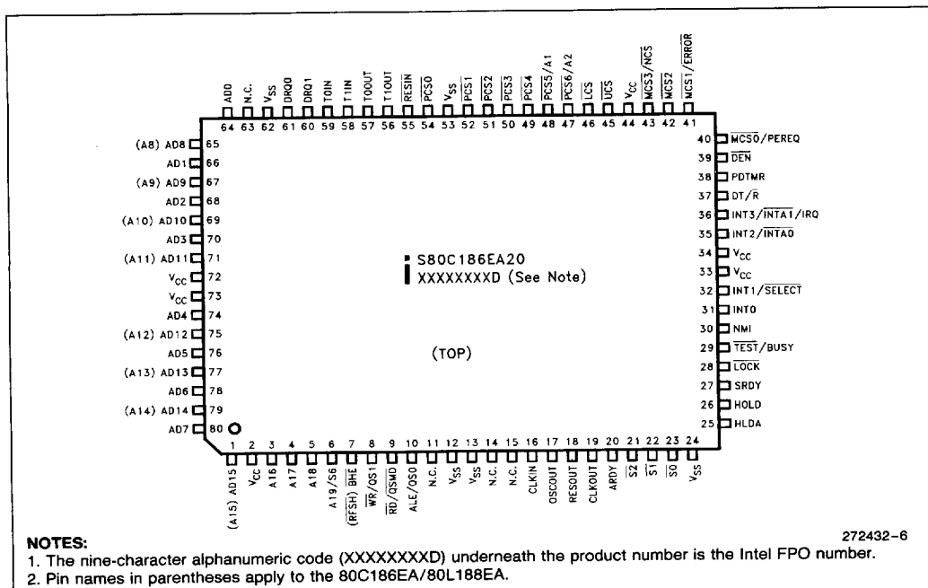
Figure 6. Quad Flat Pack (EIAJ) Pinout Diagram
