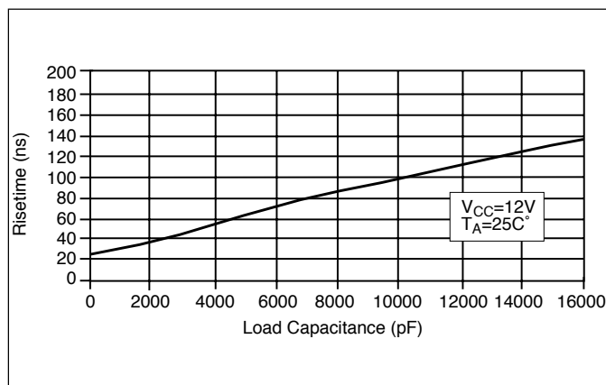
Figure 29: GATE(L) Risetime vs. Load Capacitance.
