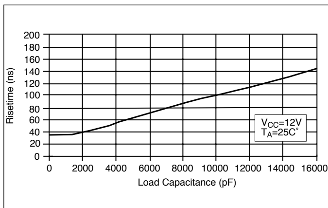
Figure 32: GATE(H) Risetime vs. Load Capacitance.
