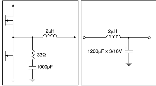
Figure 27: Filter components.
