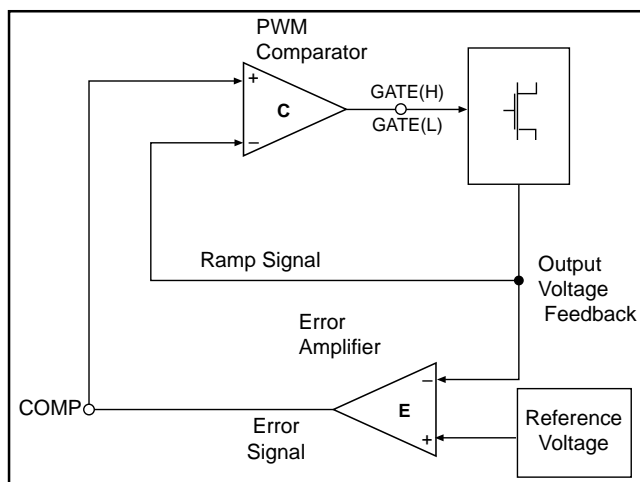
Figure 1: V 2 TM Control Diagram
