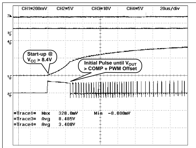
Figure 8: Normal Startup showing initial pulse followed by Soft Start (20μs/div).
