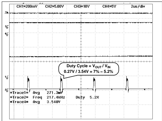
Figure 9: Pulse-by-Pulse Regulation during Soft Start (2μs/div).
