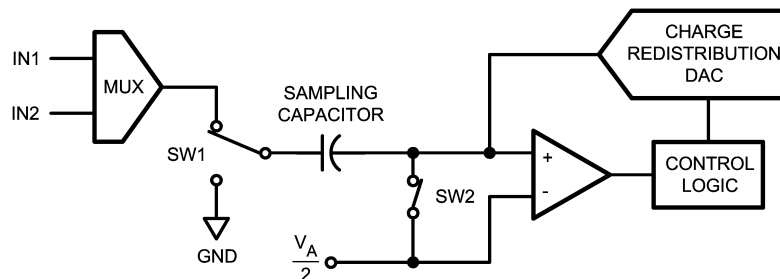
FIGURE 1. ADC082S051 in Track Mode
