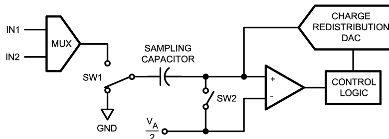
FIGURE 2. ADC082S051 in Hold Mode
