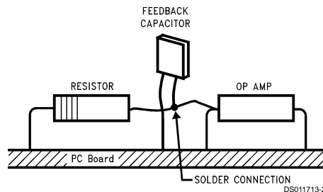
FIGURE 11. Air Wiring
