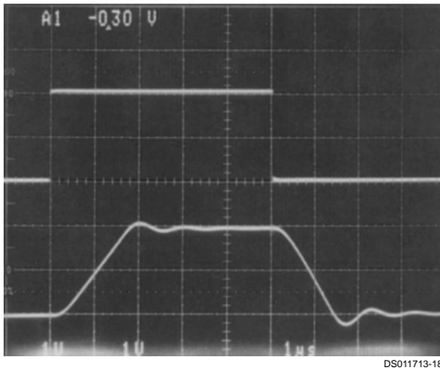
DS011713-18 FIGURE 5. Pulse Response of the LMC6482 Circuit in Figure 4
