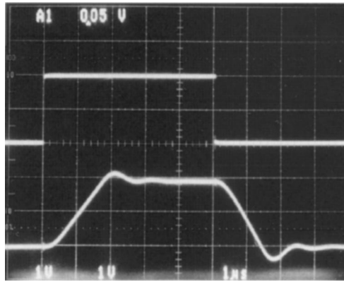
DS011713-16 FIGURE 7. Pulse Response of LMC6482 Circuit in Figure 6
