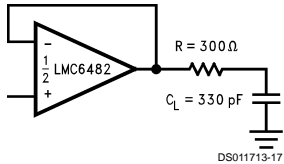
DS011713-17 FIGURE 4. Resistive Isolation of a 330 pF Capacitive Load
