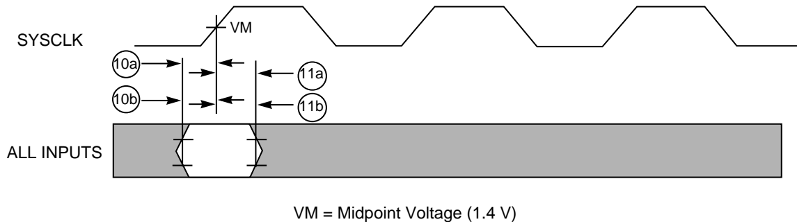
VM = Midpoint Voltage (1.4 V) Figure 2. Input Timing Diagram
