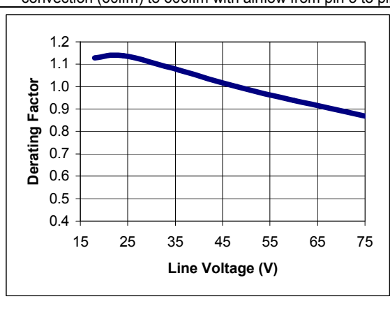
iQE4W025A033V-001 typical ambient temperature derating versus input voltage output with 1m/s (200 lfm) airflow from pin 3 to pin 1.
