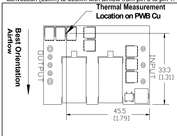
iQE4W025A033V-001 thermal measurement location – top view
