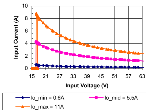
iQE4W011A120V-001 Typical Input Current vs. Input Voltage Characteristics
