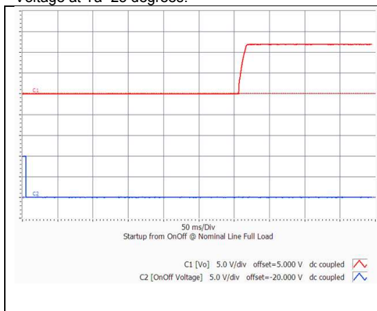
iQE4W011A120V-001 Typical startup characteristic from on/off at full load. Lower trace - on/off signal, upper trace - output voltage
