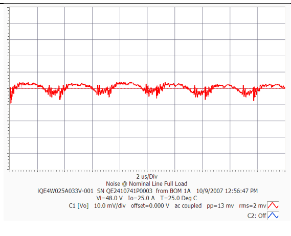
iQE4W025A033V-001 Typical Output Ripple at nominal Input voltage and full load at Ta=25 degree
