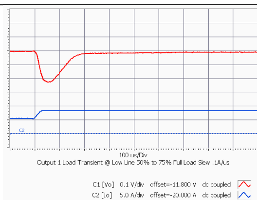
iQE4W011A120V-001 Typical transient response. Output voltage response to load step from 50% to 75% of full load with output current slew rate of 0.1A/uS.
