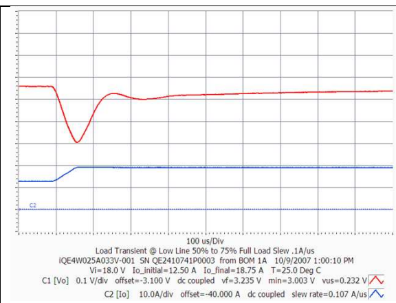
iQE4W025A033V-001 Typical transient response. Output voltage response to load step from 50% to 75% of full load with output current slew rate of 0.1A/ \mu s.
