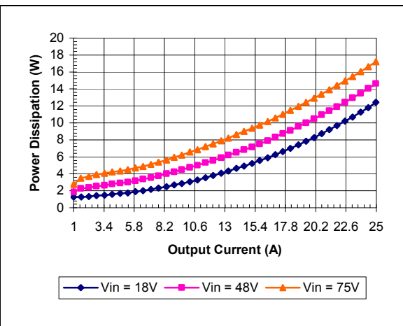
iQE4W025A033V-001 Typical Power Dissipation vs. Input Voltage at T_a = 25 degrees
