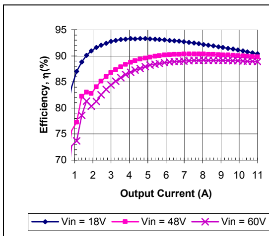
iQE4W011A120V-001 Typical Efficiency vs. Input Voltage at T_a=25 degrees.
