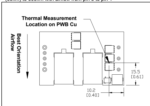
iQE4W011A120V-001 thermal measurement location – top view
