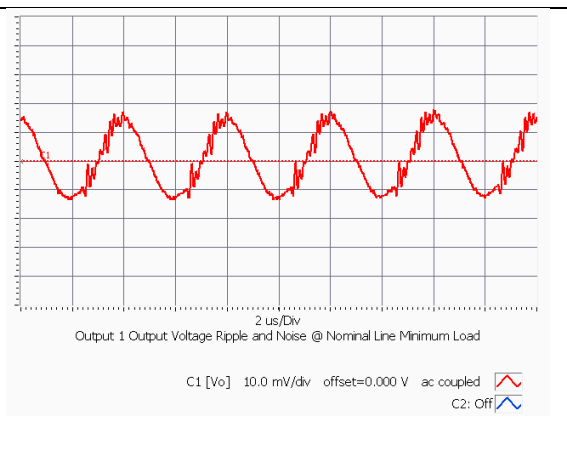
iQE4W011A120V-001 Typical Output Ripple at nominal Input voltage and full load at Ta=25 degree
