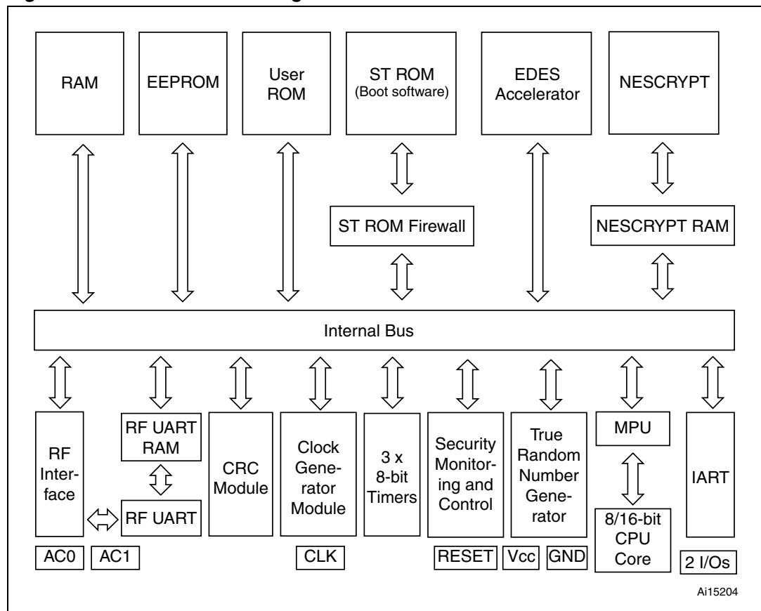
Figure 1. ST23YR48 block diagram
