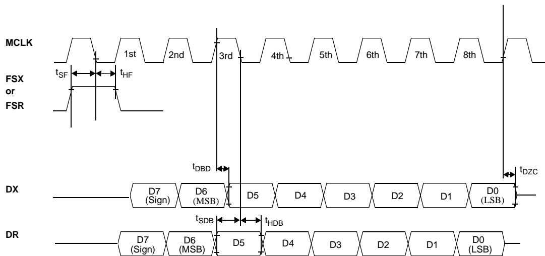
FIGURE 6. Timing diagram for PCM Interface, 8-bit mode (Short Frame Sync) for each channel
