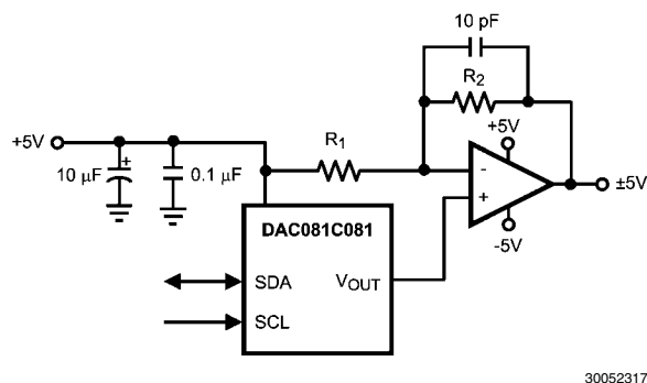
FIGURE 14. Bipolar Operation
