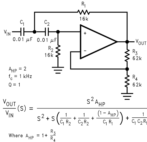
FIGURE 14. Sallen-Key 2nd-Order Active High-Pass Filter
