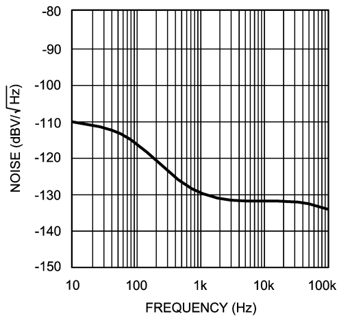
Output Voltage Noise vs. Frequency (LMV1032-15)
