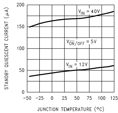
Standby Quiescent Current
