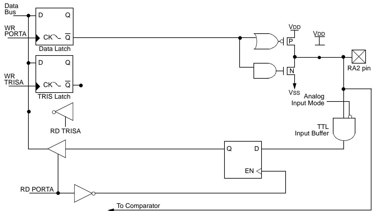
FIGURE 5-3: BLOCK DIAGRAM OF RA2/AN2/CVREF/VREF- PIN
