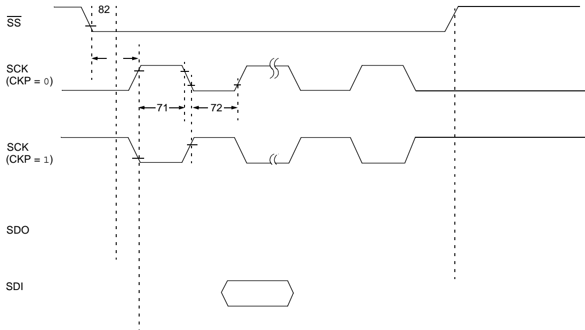
FIGURE 18-13: SPI™ SLAVE MODE TIMING (CKE = 1)
