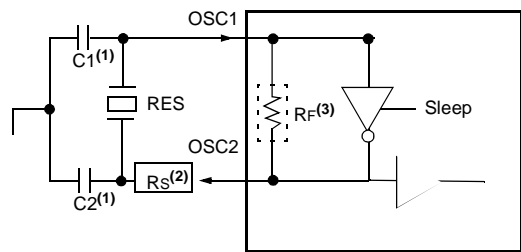
FIGURE 4-2: CERAMIC RESONATOR OPERATION (HS OR XT OSC CONFIGURATION)
