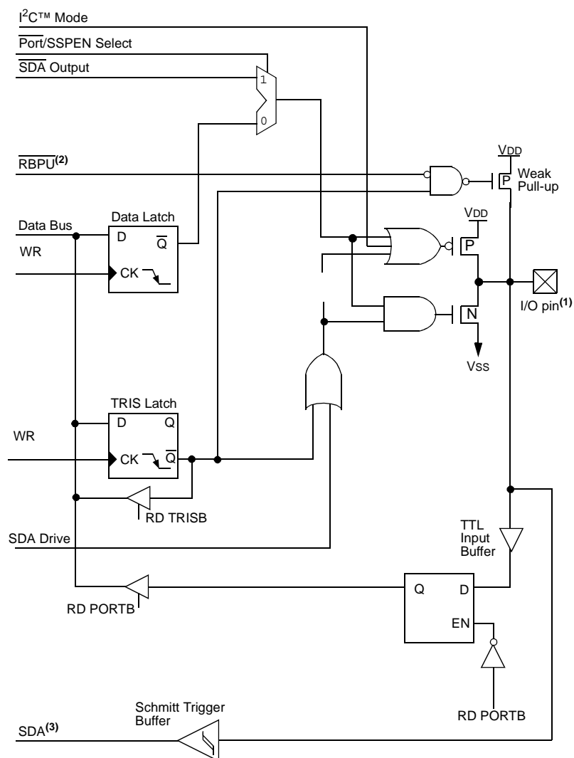
FIGURE 5-9: BLOCK DIAGRAM OF RB1/SDI/SDA PIN
