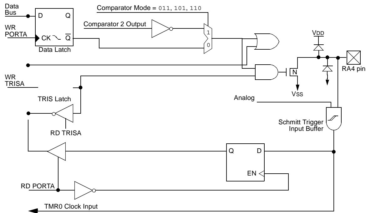
FIGURE 5-4: BLOCK DIAGRAM OF RA4/AN4/T0CKI/C2OUT PIN
