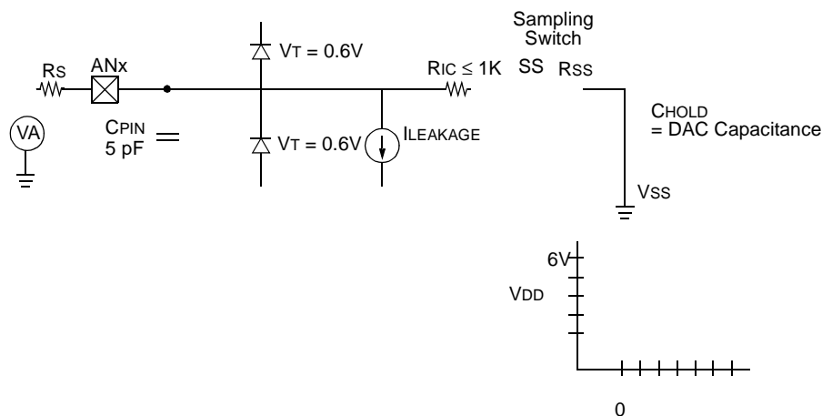
FIGURE 12-2: ANALOG INPUT MODEL
