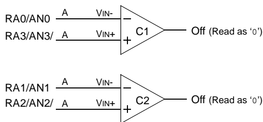
FIGURE 13-1: COMPARATOR I/O OPERATING MODES
