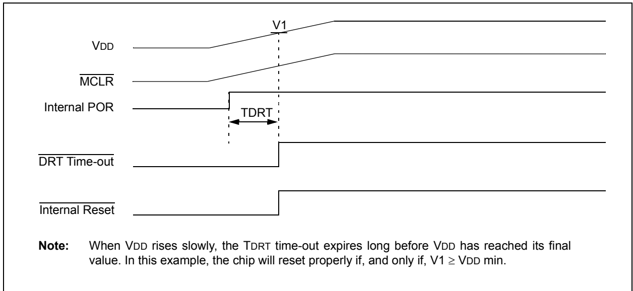
FIGURE 9-5: TIME-OUT SEQUENCE ON POWER-UP ( \overline{\text{MCLR}} TIED TO \text{V}_{\text{DD}} ): SLOW \text{V}_{\text{DD}} RISE TIME
