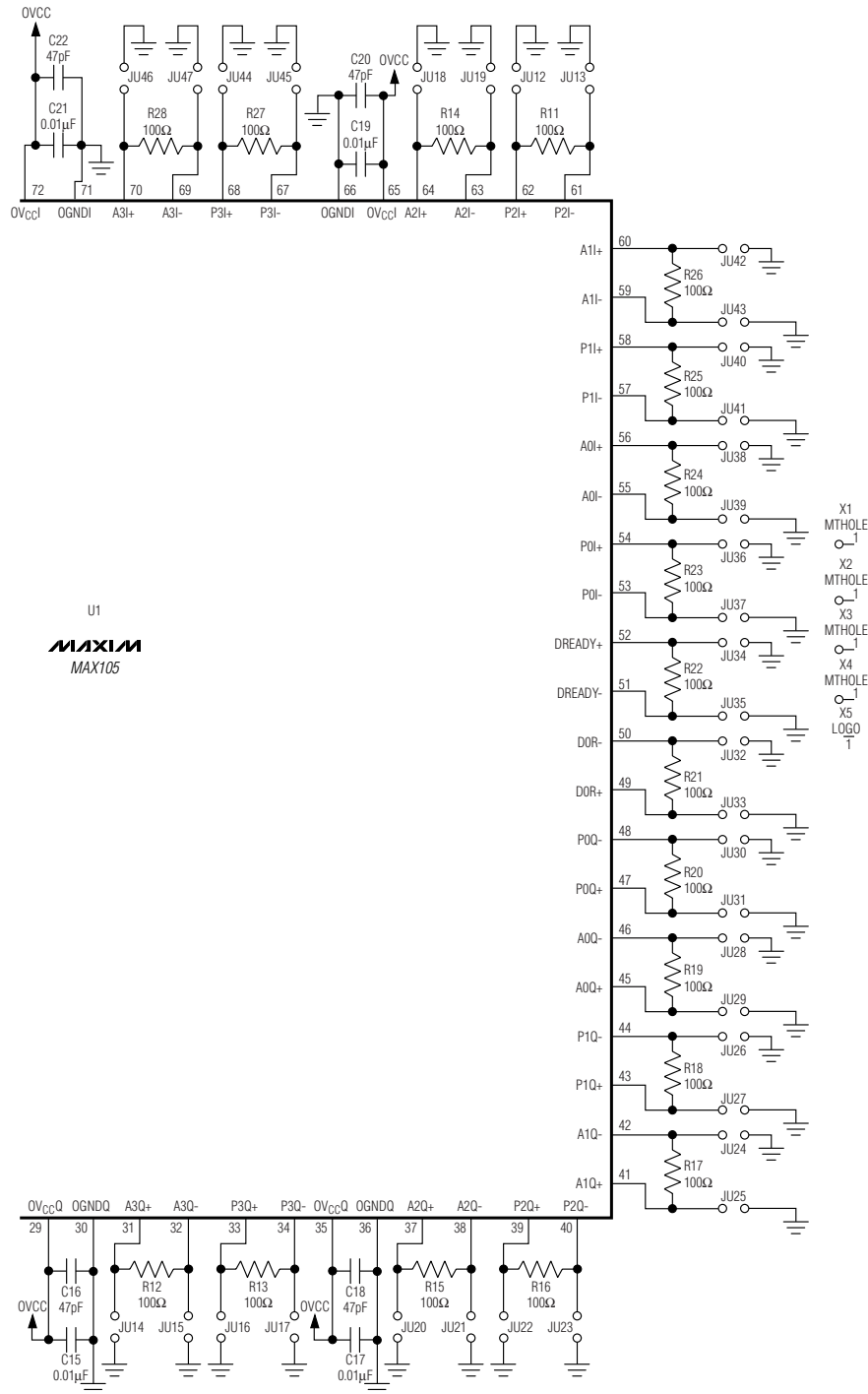
Figure 5b. MAX105 EV Kit Schematic (continued)
