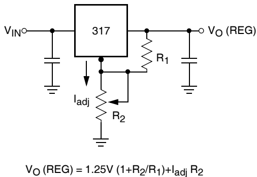
Voltage Regulator
