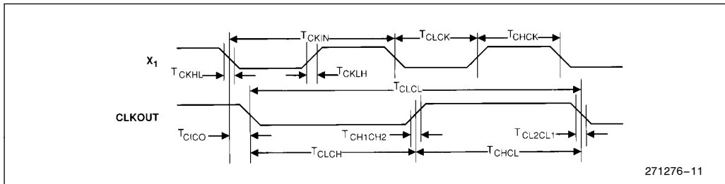
Figure 9. Clock Waveforms
