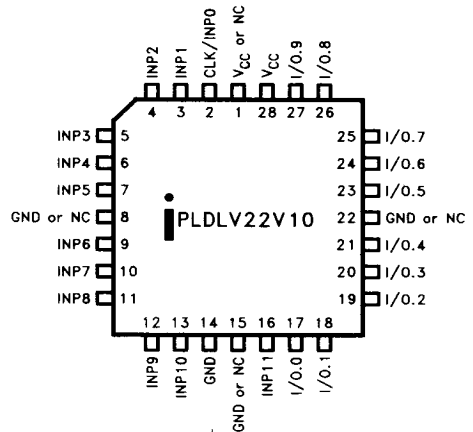
Figure 1. Pinout Diagrams
