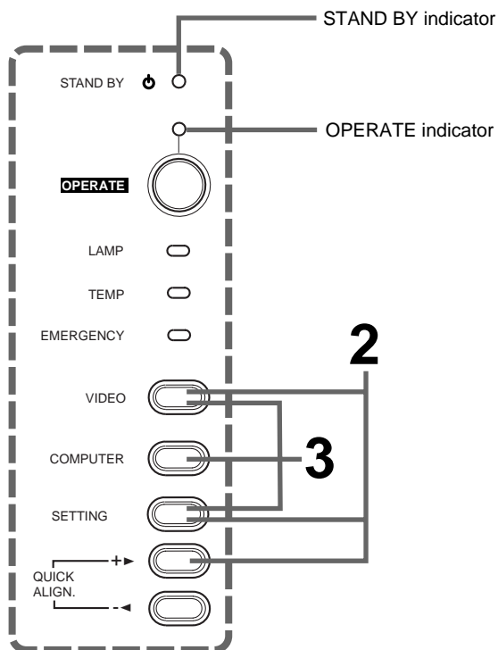
[Control panel]
