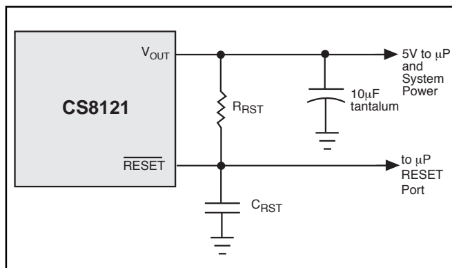
Figure 4. RC Network for \overline{\text{RESET}} Delay
