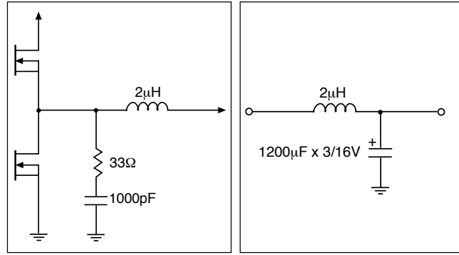
Figure 27: Filter components.
