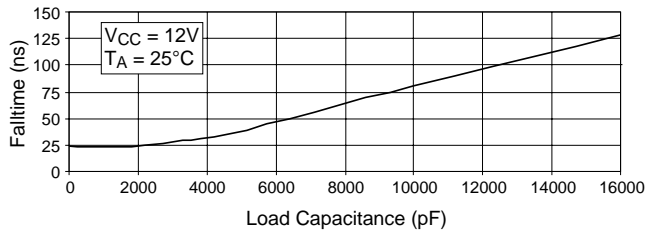
Figure 1: Gate(H) and Gate(L) Faltime vs. Load Capacitance.
