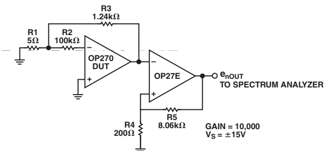
Figure 9. Current Noise Density Test Circuit
